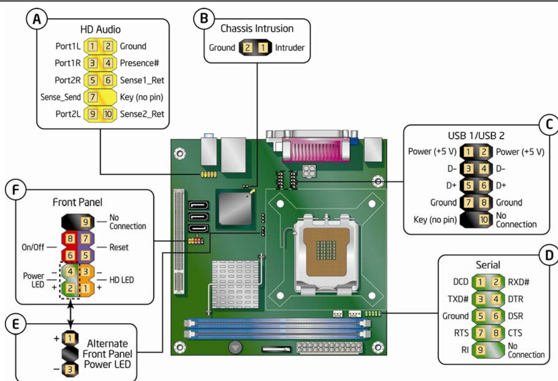
Figure 18. Internal Headers and Connectors
