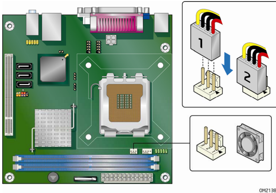
Figure 20. Location of the Chassis Fan Header
