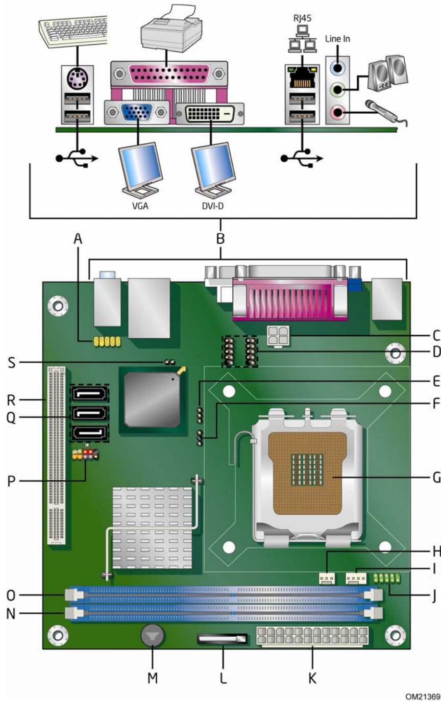
Figure 1. Intel Desktop Board DG41MJ Components
